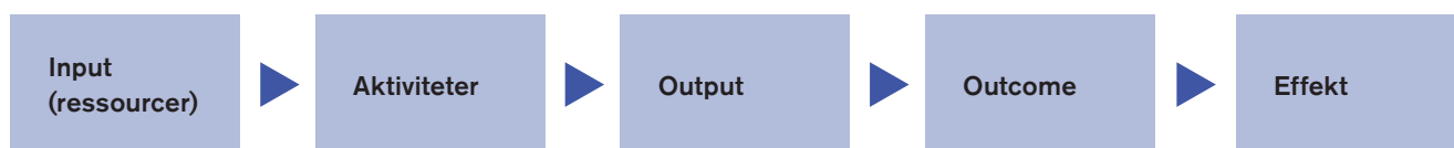
Figur 5: Input-output-model
